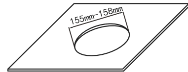
Installation Hole
