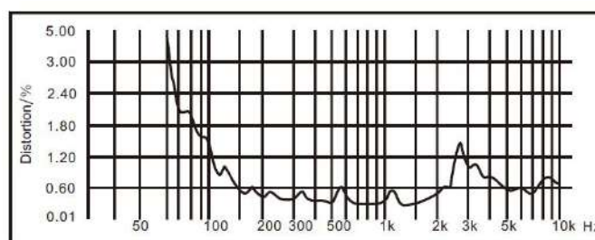
Distortion Characteristics (THD< 3% 1W, 1m, 100Hz-10kHz)
