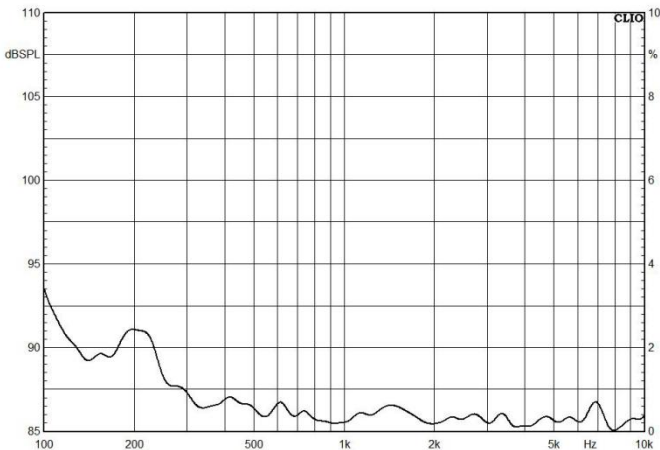
Distortion (% THD, 1W, 1m)
